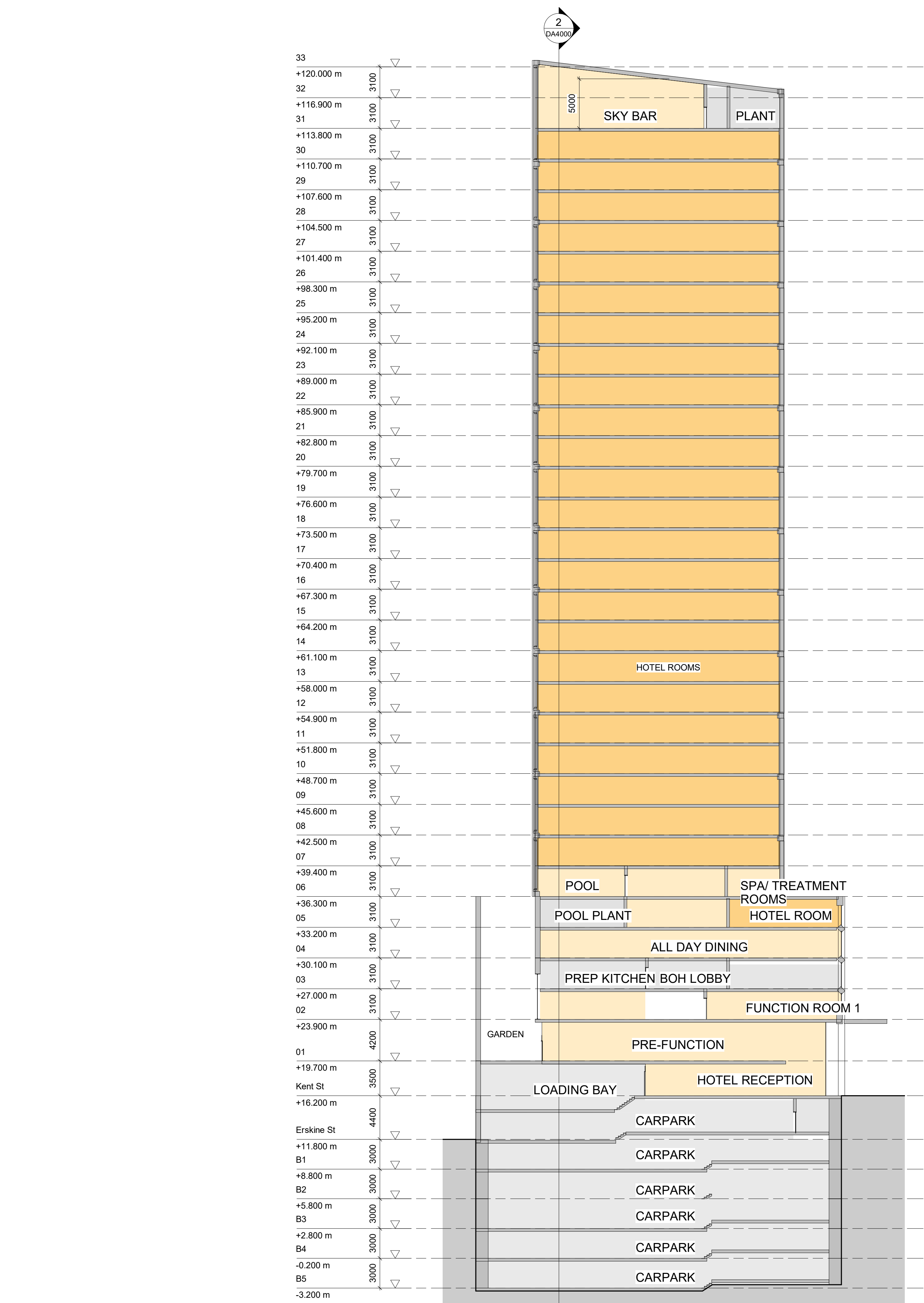
1 BUILDING SECTION - EAST/ WEST 1 : 250 REF:1/A2250
