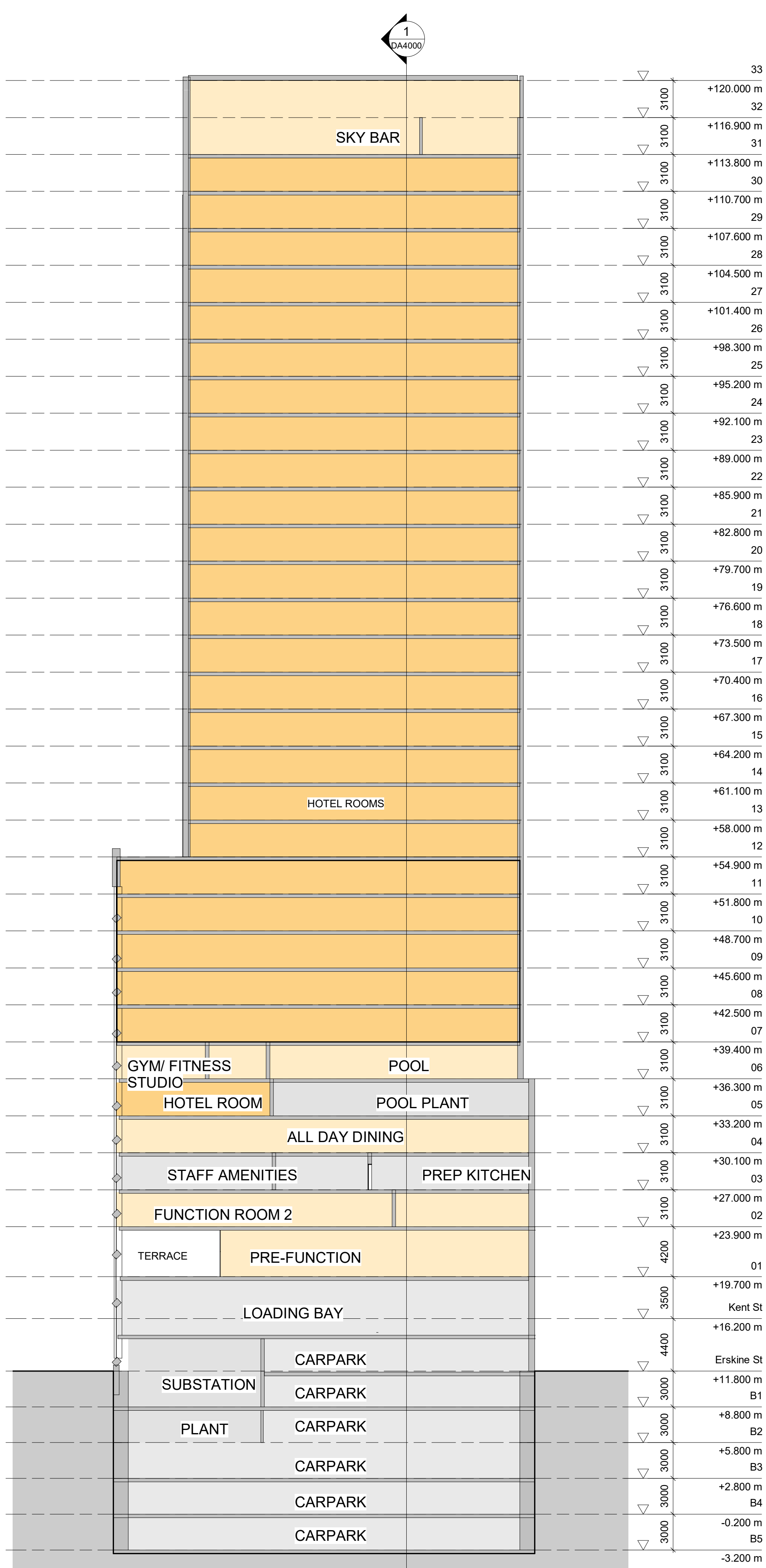
2 BUILDING SECTION - NORTH/ SOUTH 1 : 250 REF:2/A2250
